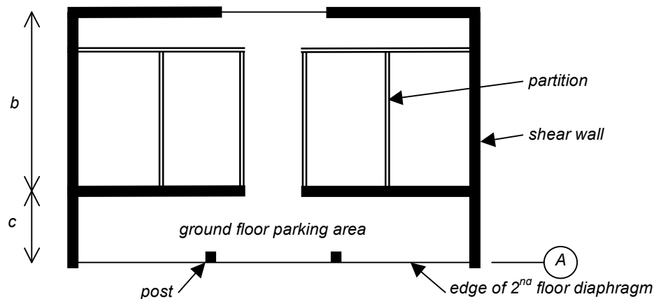
Figure C4-1. Excessive cantilever calculation.
