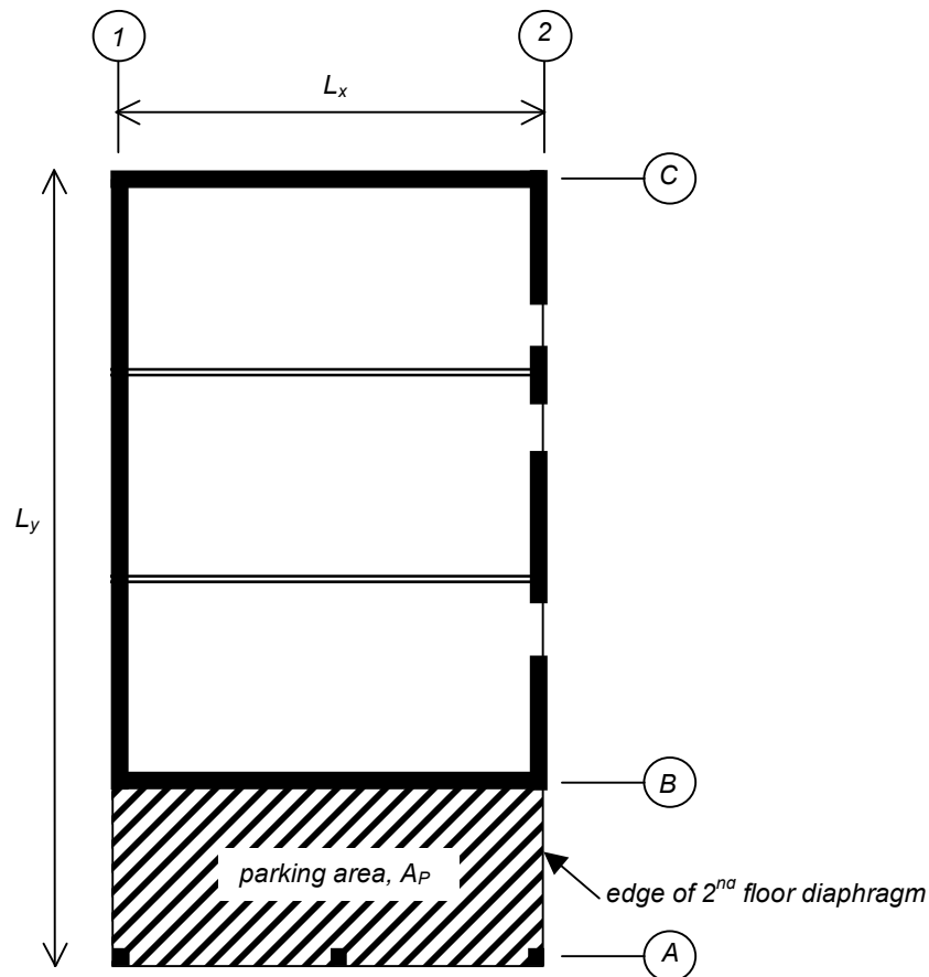
Figure C4-2. 20 percent exception calculation.
